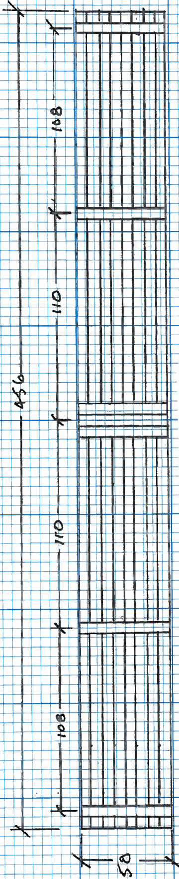
BOTTOM VIEW
