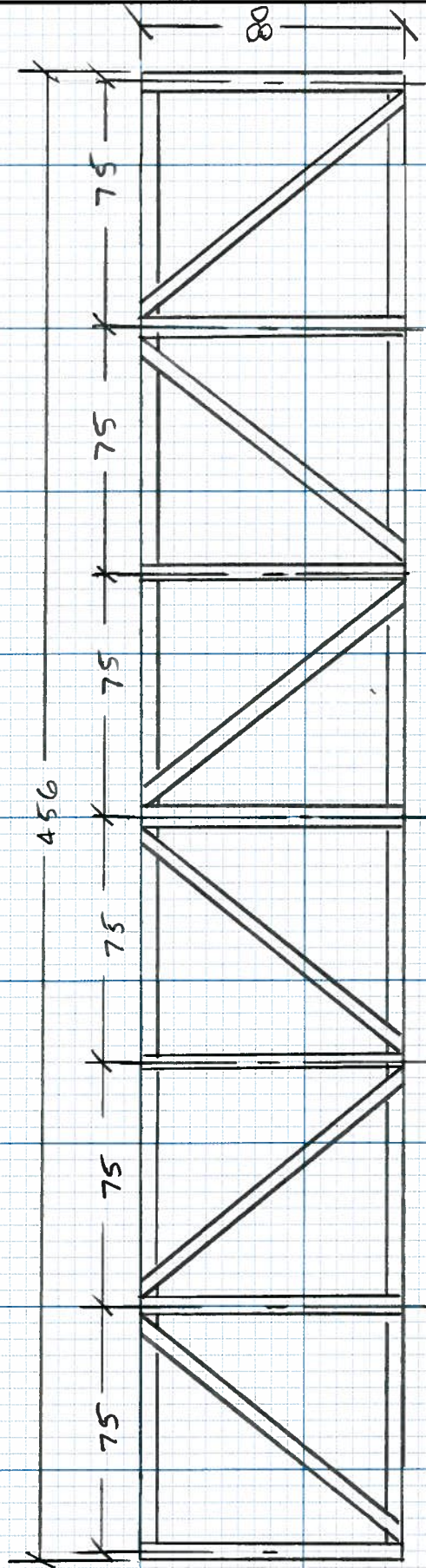
ELEVATION WITH FRONT RAILS REMOVED TO SHOW JOINT DETAILS
